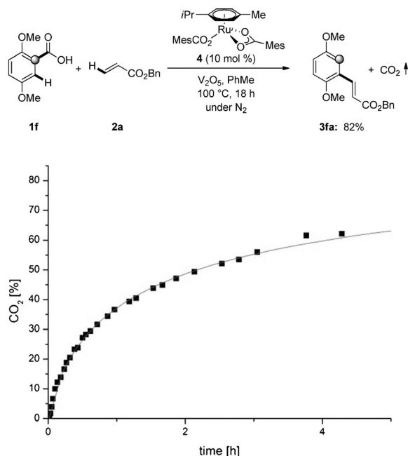
Figure 2. CO 2 evolution during ruthenium(II)-catalyzed C–H alkenylation.
