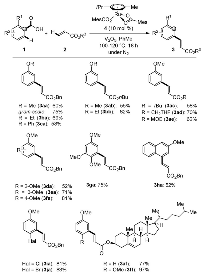
Scheme 1. Scope of the decarboxylative domino C–H alkenylation with benzoic acids ( 1 ) and alkenes ( 2 ). THF = tetrahydrofuran-2-yl, MOE = 2-methoxyethyl.
