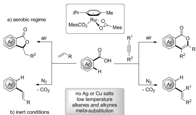
Figure 1. Ruthenium(II)-catalyzed decarboxylative C–H olefination.
