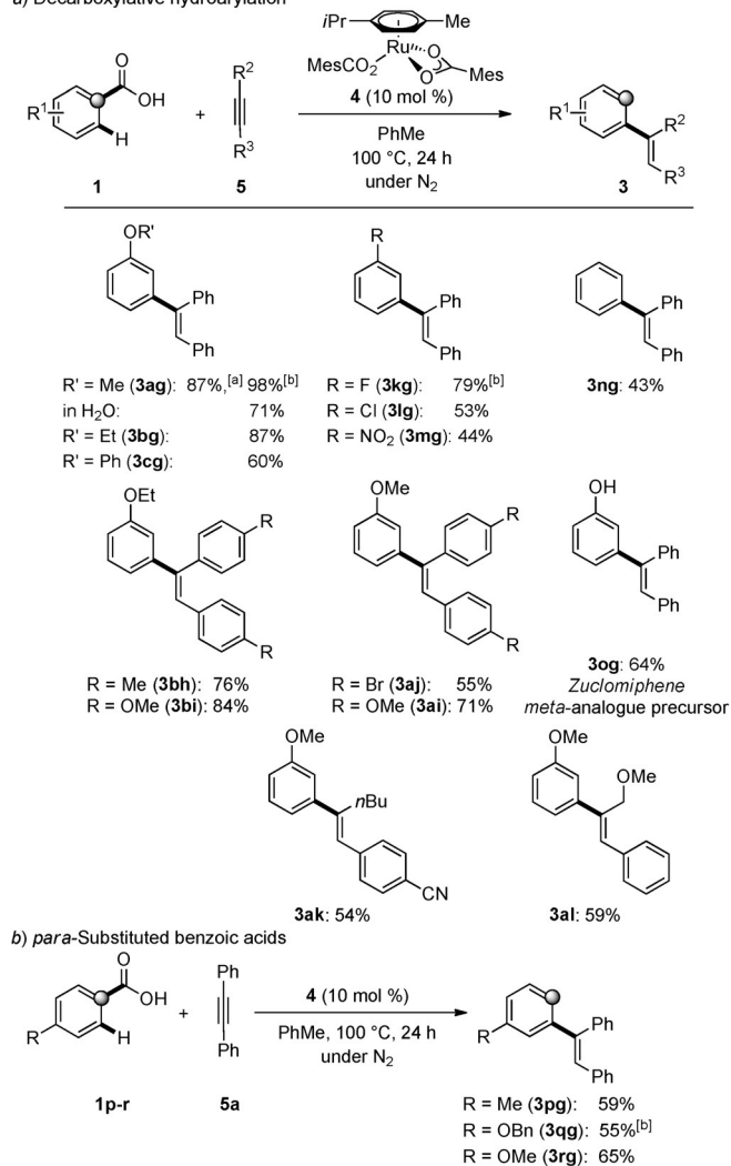
Scheme 2. Decarboxylative hydroarylation.[a] 4 (5.0 mol%). [b] In DCE.
